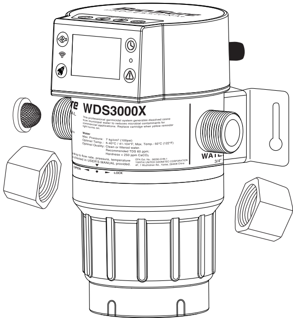
Main Device [ attachments include Ozone Generator Cartridge (x1) and Connector Caps (x4) and Inlet Screen Filter (x1) ]
